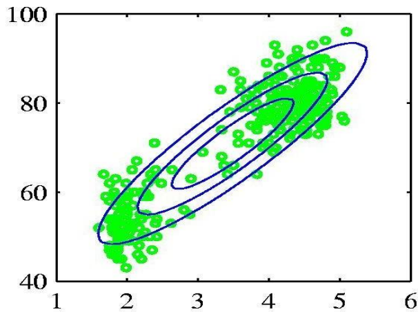
Single Gaussians
