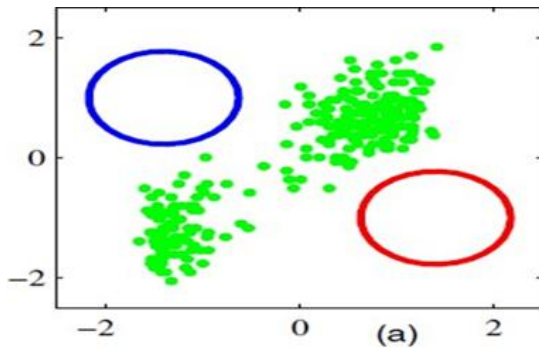
Initialization
