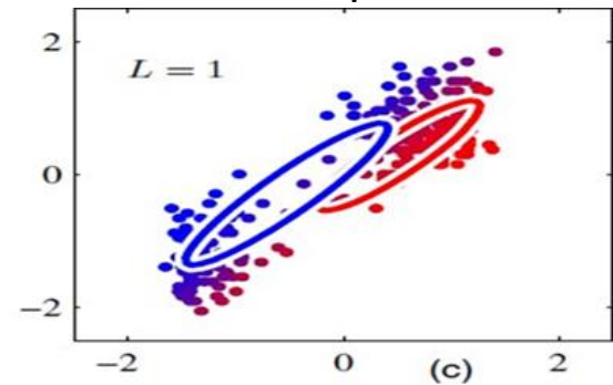
M Step
